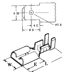
250 FLAT REC for single-pole
