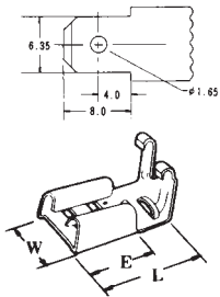
250 FLAT FLAG REC for single-pole
