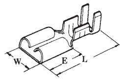
250 FLAT lance-less REC for multi poles
