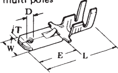
250 FLAT TAB for multi poles
