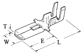
250 FLAT lance-less TAB for multi poles
