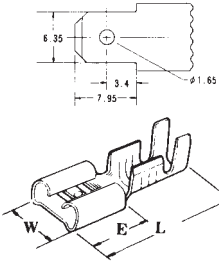
250 FLAT REC with window for single-pole
