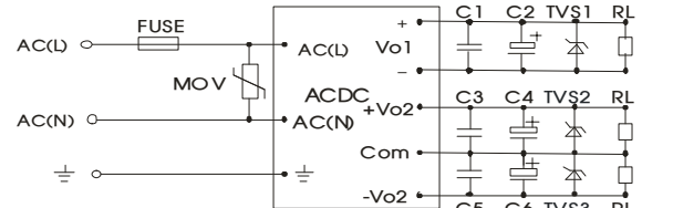
Fig. 4: LH15-10Cxx (Triple Output) series typical application circuit
