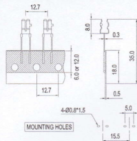
CQ-216 HOT For 10.3mm Dia. Fuse
