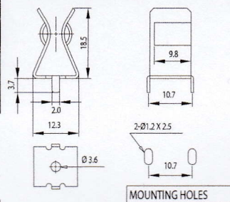
CQ-216(G) For 10.3mm Dia. Fuse
