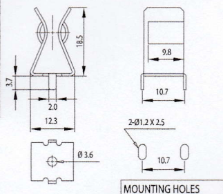
CQ-216 HOT For 10.3mm Dia. Fuse
