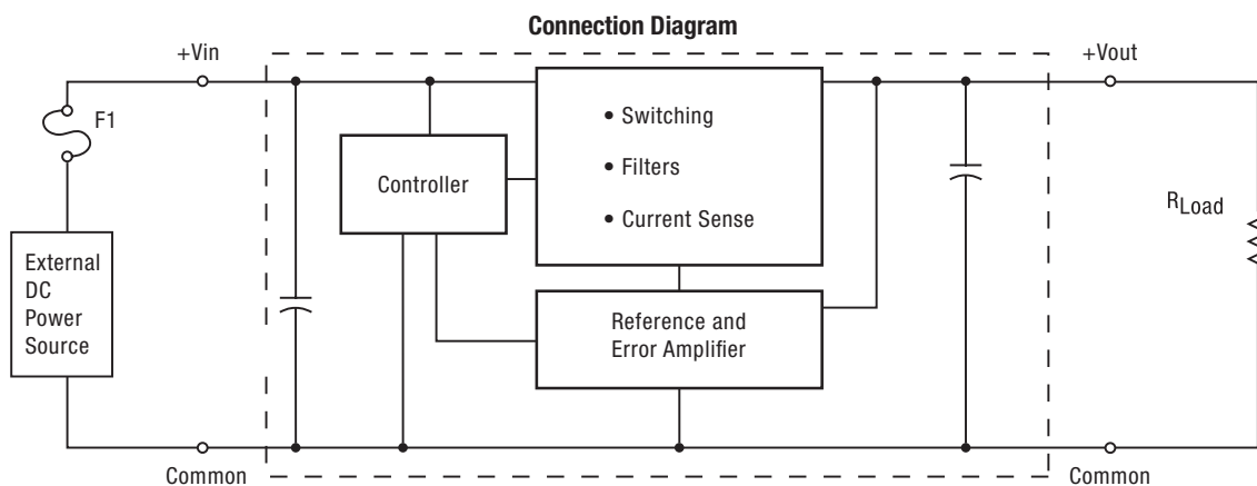
Figure 1. OKI-78SR
