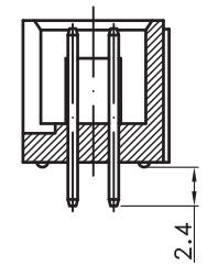
(DIP 2.4mm)
