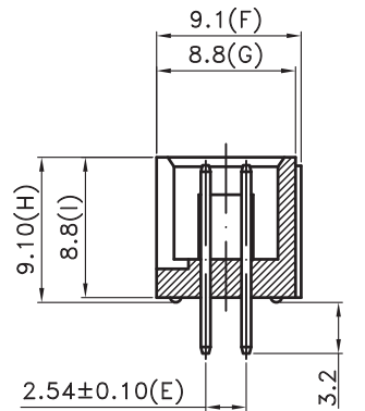
(DIP 3.2mm Standard)
