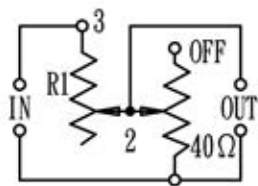
CIRCUIT
