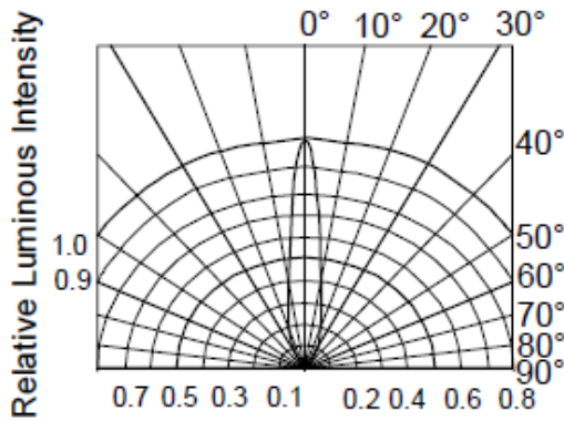
RADIATION DIAGRAM
