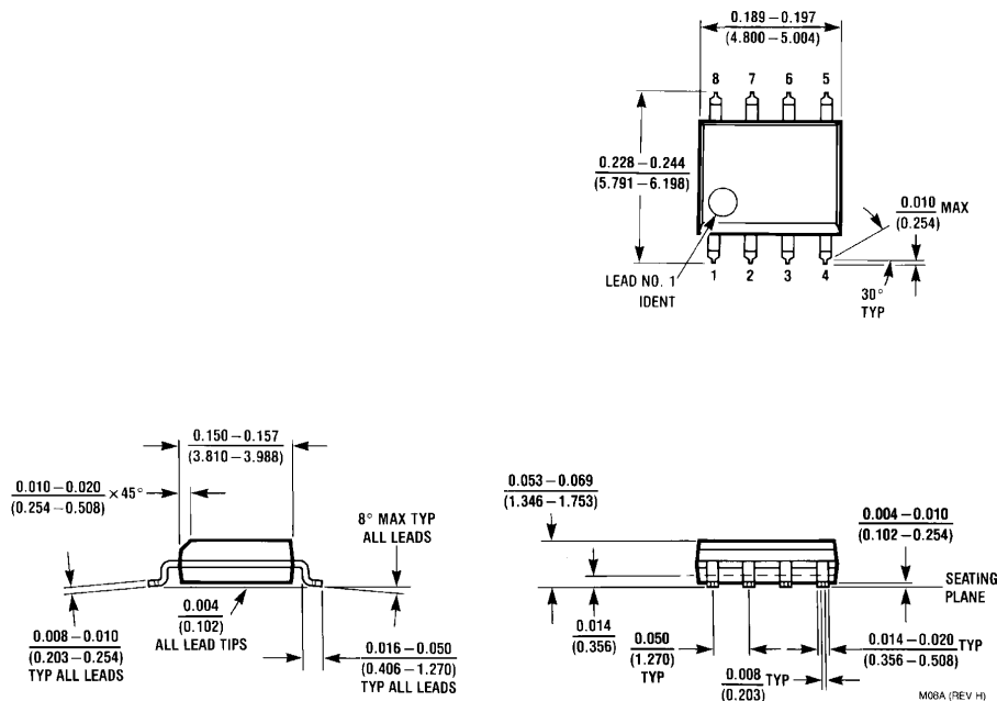
Order Number LM4881M NS Package Number M08A
