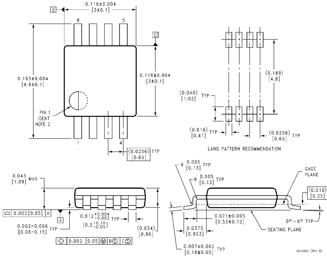
Order Number LM4881MM NS Package Number MUA08A
