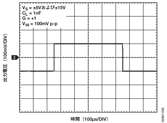
図33. 小信号過渡応答
