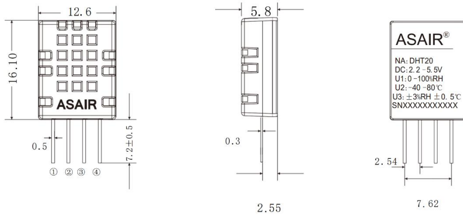
Figure 13. DHT20 sensor encapsulation (unit: mm not specified tolerance: ± 0.2 mm)
