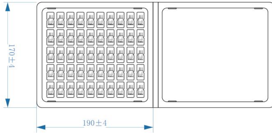
Figure 12. DHT20 sensor package diagram (unit: mm unmarked tolerance: ± 0.2mm)
