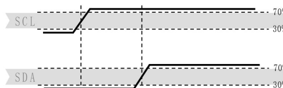
Figure 11. Stop transmission state (P)
