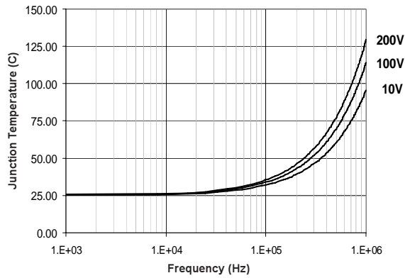
Figure 33. IR2010S Tj vs Frequency R_{GATE} = 16 \text{ Ohm}, V_{cc} = 15V \text{ with IRFBC40}
